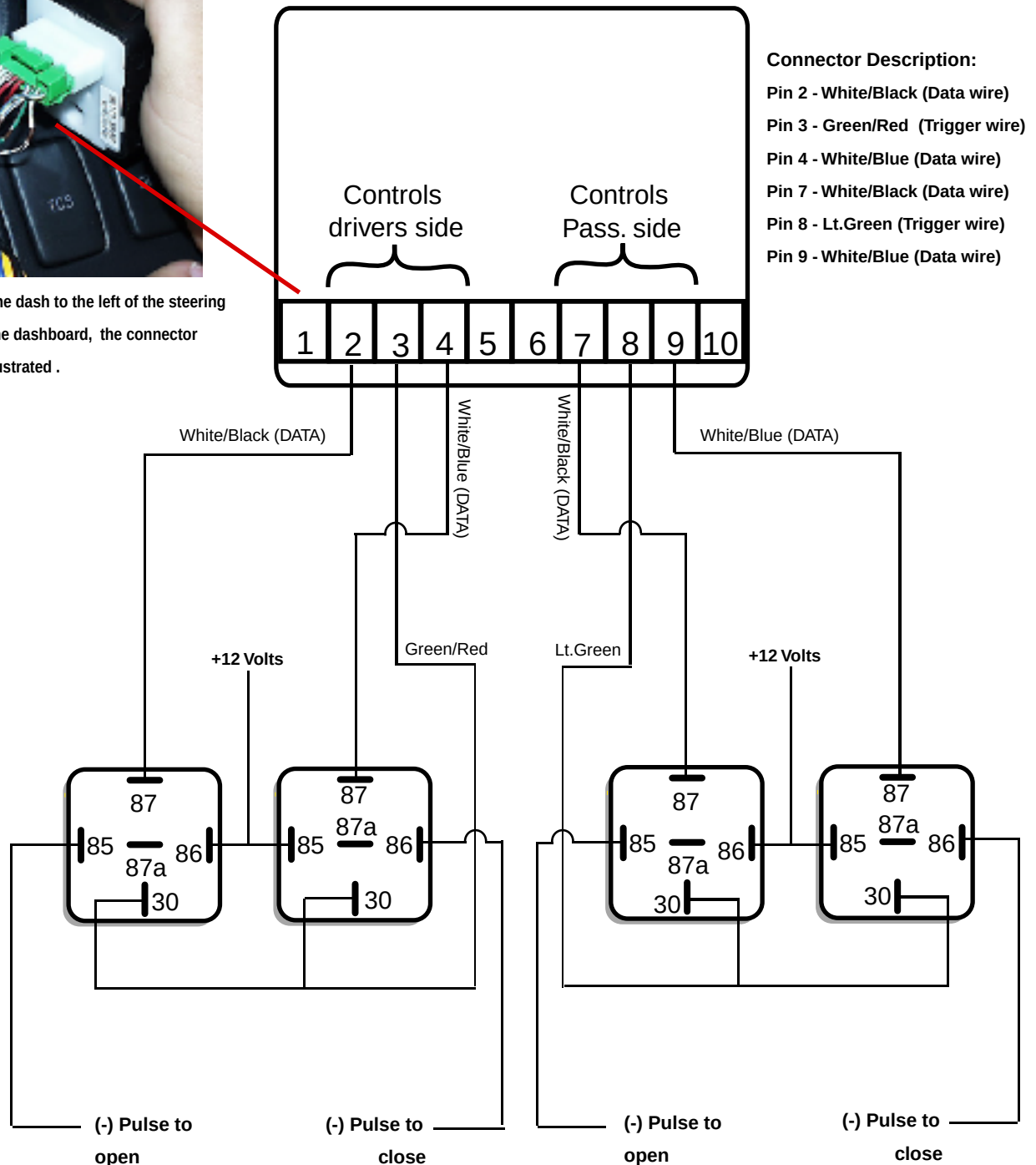
Rear view of door control switch
